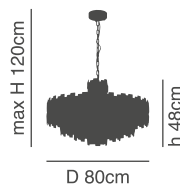
77-8209-662 M6603-800 16xE14, max 40W, 230V
