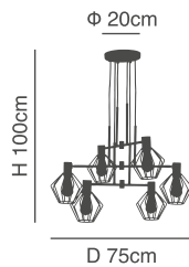
77-8877-214 SE21-BL-100-GR1 6xE27, max 60W, 230V
