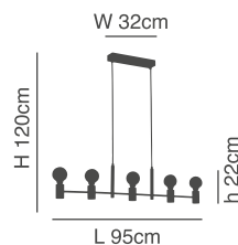
77-8249-123 SE21-BL-120 5xE27, max 60W, 230V
