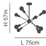
77-8096-78 KQ 2629/8 8xE27, max 60W, 230V
