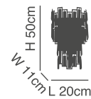
77-8211-104 M8021G 2xE14, max 40W, 230V
