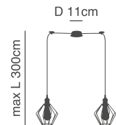
77-8706-63 SE21-BR-10-BL2-GR1 2xE27, max 60W, 230V
