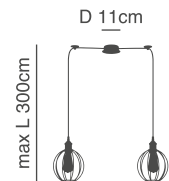
77-8713-63 SE21-BR-10-BL2-GR2 2xE27, max 60W, 230V
