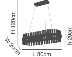
77-8213-276 M6612-800R LED, 72watt, 5400lumen, 230V
