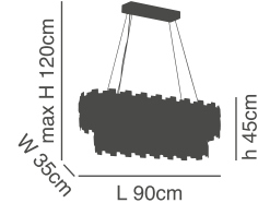
77-8210-533 M6603-900R 10xE14, max 40W, 230V
