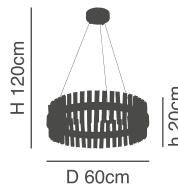
77-8212-212 M6612-600 LED, 67watt, 5025lumen, 230V
