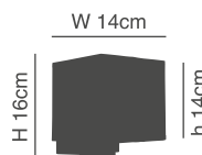
77-3559-31 SE-120-1A 1xE14, max 40W, 230V
