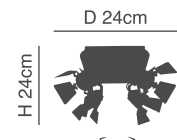
77-2211-148 GU12015A-4R 4xGU10, max 50W, 230V
