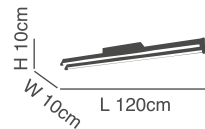
77-1796-23 MB-095 2x54W, T5, 230V
