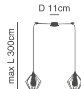
77-8749-51 SE21-BL-B10-BL2-GR1 2xE27, max 60W, 230V
