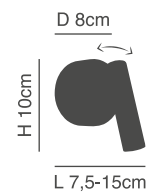
77-3518-25 SE-127-1AB LED, 1xE27, 3W, 230V
