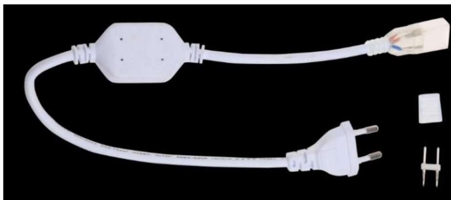
LED DRIVER PARA TIRA DE 220V 50 METROS REF PB22050 AC220-240V 50/60Hz DC198-216V MAX WATTIOS 400W
